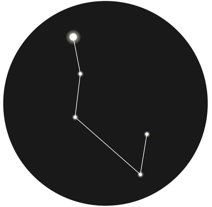
Lyra
